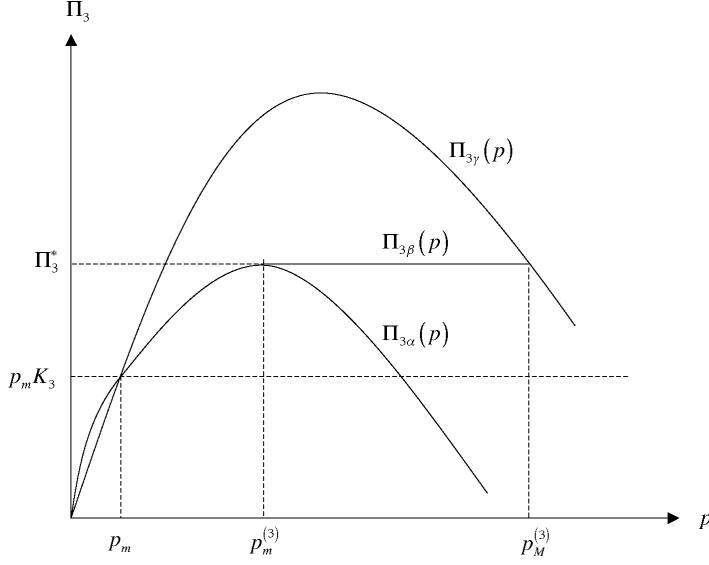
Fig. 2 \Pi_{3\alpha}(p) := Z_3(p, \phi_{1\alpha}(p), \phi_{2\alpha}(p)) , where p_m K_1 = Z_1(p, \phi_{2\alpha}(p), 0) and p_m K_2 = Z_2(p, \phi_{2\alpha}(p), 0) ; \Pi_{3\gamma}(p) := Z_3(p, \phi_{1\gamma}(p), \phi_{2\gamma}(p)) , where p_m K_1 = Z_1(p, \phi_{2\gamma}(p), 1) and p_m K_2 = Z_2(p, \phi_{2\gamma}(p), 1)
