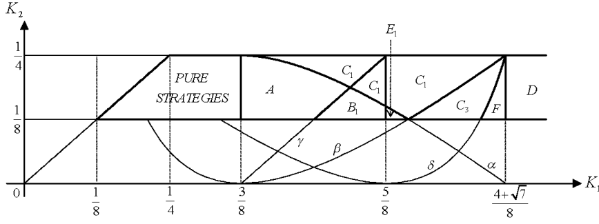
Fig. 1 Taxonomy for D(p) = 1 - p and K_2 + K_3 = 1/4 .
